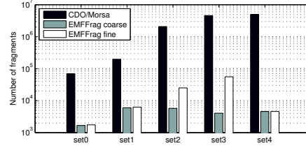
Fig. 12. Number of fragments used by the different persistence frameworks.
