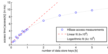
Fig. 4. HBase accesses performance.
